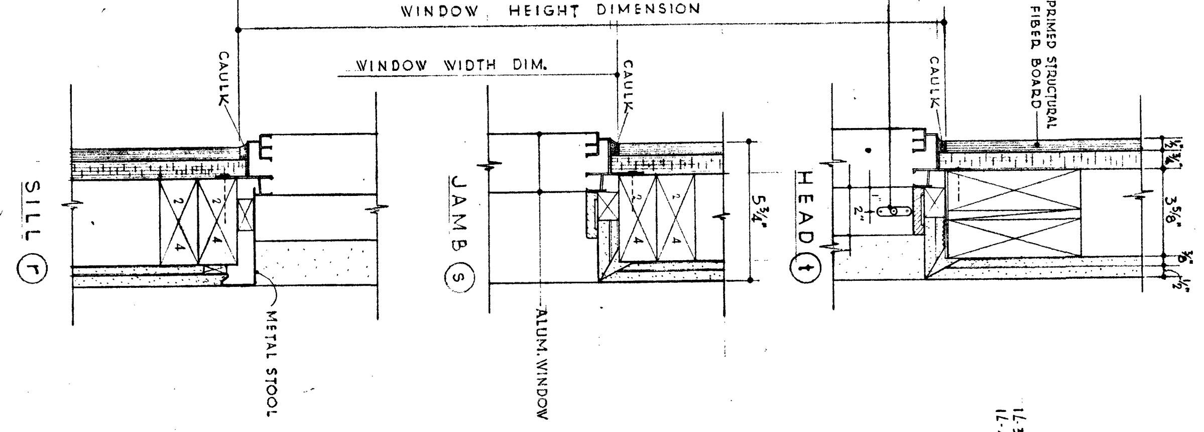
WINDOW DETAILS SCALE 3/4" = 1'-0"
